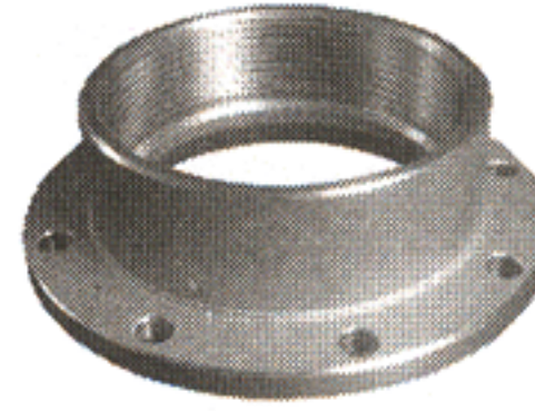
TTFNPTF TTMA Flange X Female NPT Made in U.S.A.
