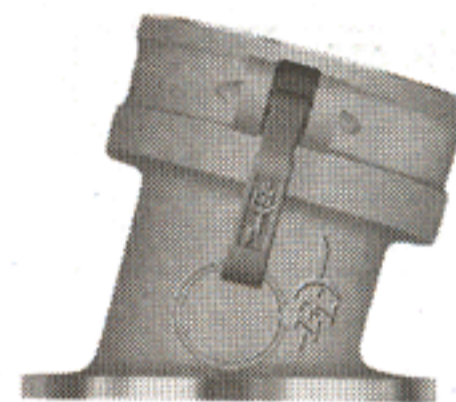
Part TTF40C-15 Coupler X Tank Truck Flange 15° Made in U.S.A.
