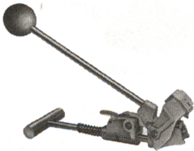
P-1000™ Loking Tool "The Punch-Lok Tool" The original. Made like no other tool! Designed for fast, economical application of punch-type clamps. The portable P-1000 weighs only 2 1/2 pounds. Drop forged and double plated tempered steel construction.
