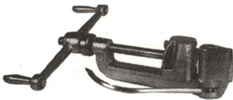
PB-001 Banding Tool Forged double plated tensioning tool with built-in cutter for banding and buckle application. Also can be used with PJ-001 for J-Lok Clamp installation.
