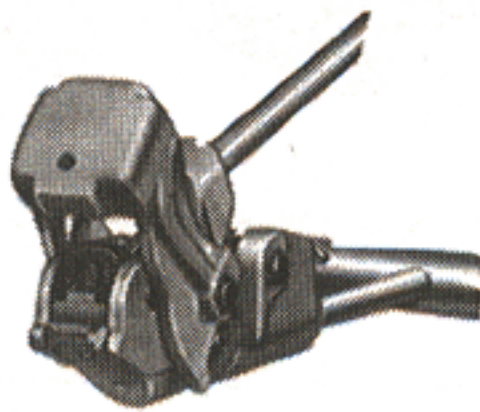
P-3000™ Loking Tool Similar to the Model P-1000, the Model P-3000 is for application of 3/8" wide punch-type clamps only. It will not fit 5/8" wide clamps. Double plated.
