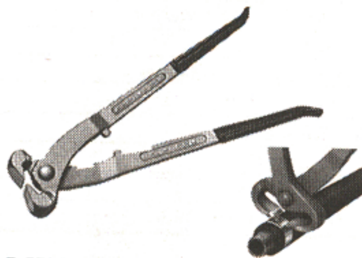
D-550™ Clamp Cutter Powerful 14" cutter removes any punch-type clamp with minimum effort. Rugged drop forged heat treated high-carbon steel construction. Double plated. "All New Design"
