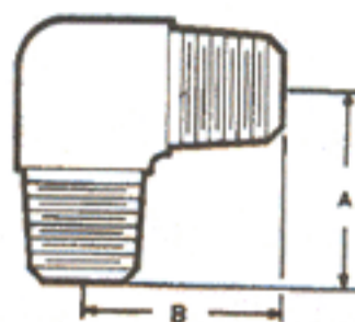
A169 Series 90 Degree Male Pipe Nipple NPTF - Dryseal
