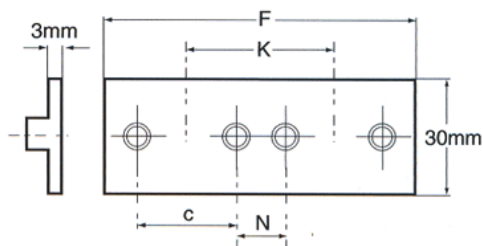
DOUBLE WELD PLATE
