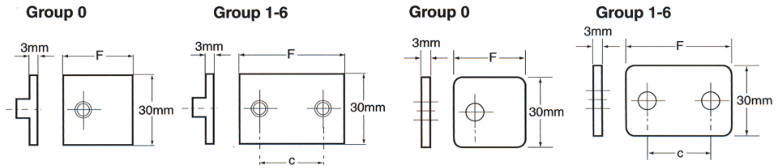
WELD PLATE
