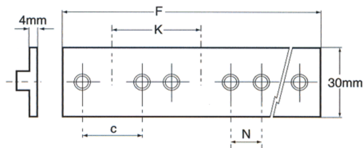
MULTIPLE WELD PLATE
