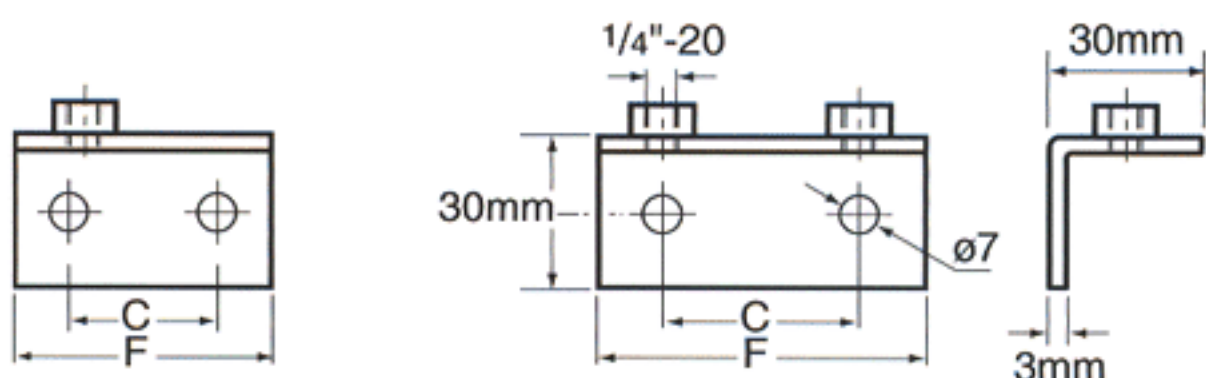
ANGLED WELD PLATE
