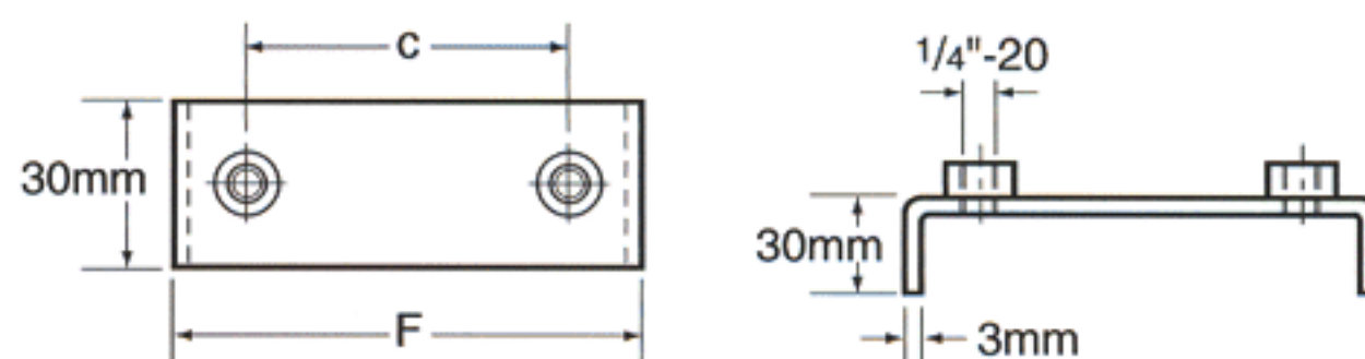
BRIDGE WELD PLATE
