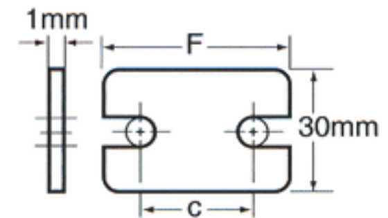
SAFETY PLATE
