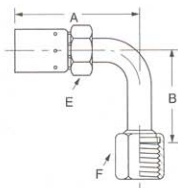
Female FOR-SEAL® Swivel Long Drop 90° Tube Elbow
