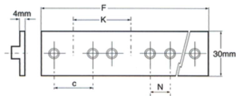
MULTIPLE WELD PLATE
