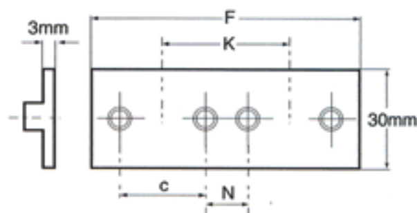
DOUBLE WELD PLATE
