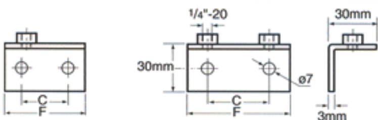
ANGLED WELD PLATE
