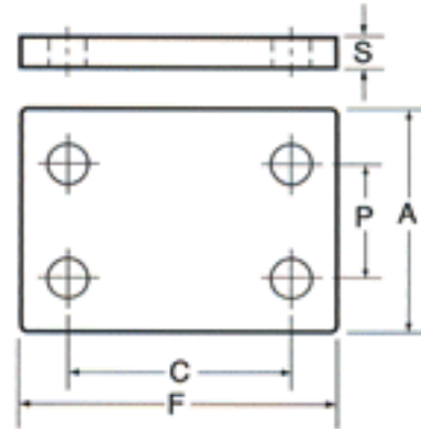
DOUBLE COVER PLATE
