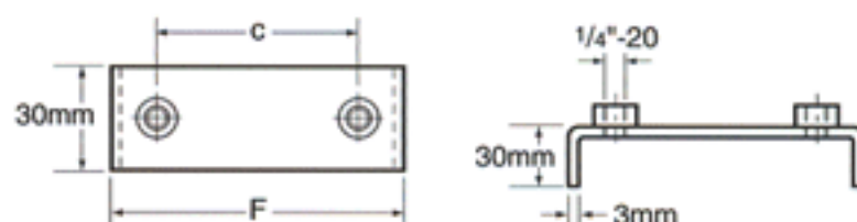
BRIDGE WELD PLATE
